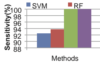
Figure 13: Sensitivity results from the comparison between classifiers
