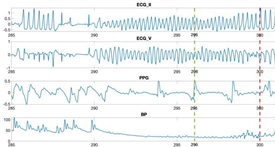
Figure 3 The figure shows the plot of recording f563I between 285 and 301 s. The figure for this recording then compares the latency of bedside monitors and that of proposed system in alerting for ventricular fibrillation. The bedside monitor identifies the presence of ventricular fibrillation at 300th s, as visualized by the red dashed line. On the other hand, the proposed system can identify the presence of ventricular fibrillation at 296th s itself (4 s earlier), as visualized by the green line.
