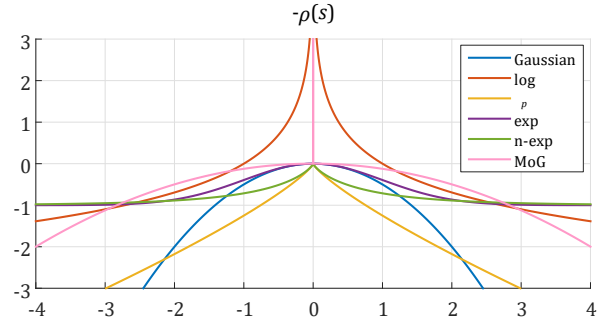
Fig. 1. Set of considered \rho(s) functions from Table 1.
