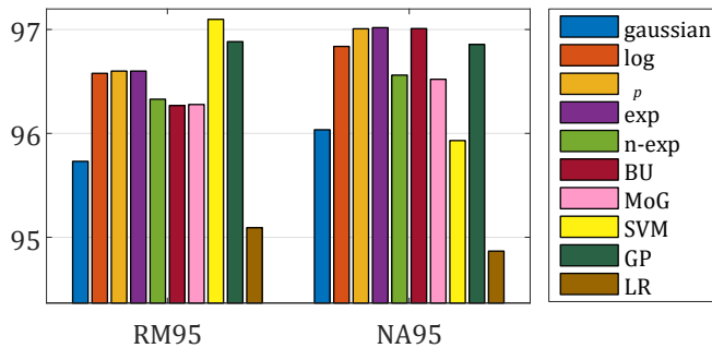
Fig. 4. Overall accuracy for different classification methods on “Rome95” and “Naples95” images.
