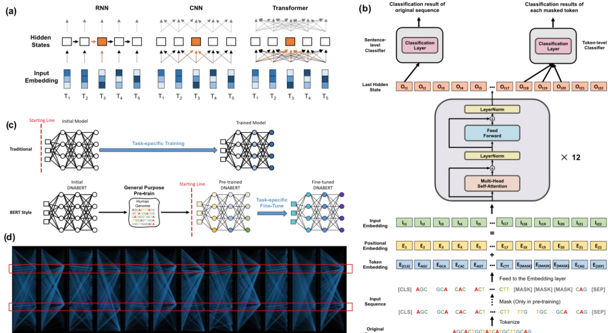
Fig. 1. Details of architecture and characteristics of DNABERT model.(a) Differences between RNN, CNN and Transformer in understanding contexts. T1 to 5 denotes embedded tokens which were input into models to develop hidden states (white boxes, orange box is the current token of interest). RNN propagates information through all hidden states, and CNN takes local information in developing each representation. In contrast, Transformers develop global contextual embedding via self-attention. (b) DNABERT uses tokenized k-mer sequences as input, which also contains a CLS token (a tag representing meaning of entire sentence), a SEP token (sentence separator) and MASK tokens (to represent masked k-mers in pre-training). The input passes an embedding layer and is fed to 12 Transformer blocks. The first output among last hidden states will be used for sentence-level classification while outputs for individual masked token used for token-level classification. Et, It and Ot denote the positional, input embedding and last hidden state at token t, respectively. (c) DNABERT adopts general-purpose pre-training which can then be fine-tuned for multiple purposes using various task-specific data. (d) Example overview of global attention patterns across 12 attention heads showing DNABERT correctly focusing on two important regions corresponding to known binding sites within sequence (boxed regions, where self-attention converged) where high quality data with labels is expensive and timeconsuming to obtain.
